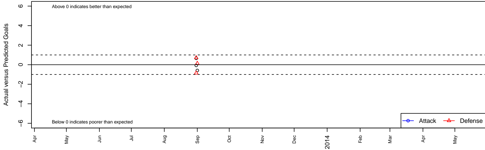
Blackhills FC Black B94 Dots are actual minus expected GF (blue circles) and GA (red triangles). Blue line is smoothed change in attack strength. Red is smoothed change in defense strength.
